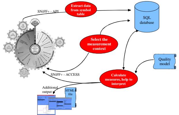
figure 6: Connection between Crocodile and SNIFF+
