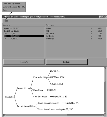
figure 9: Crocodile's quality model viewer
