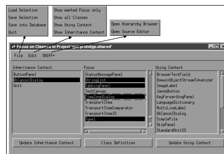
figure 8: Crocodile's context definition tool
