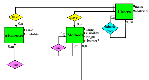
figure 2: Necessary data for measuring OO-designs
