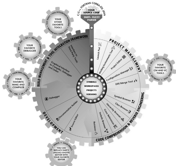
figure 5: Structure of SNIFF+ (from [Take96])
