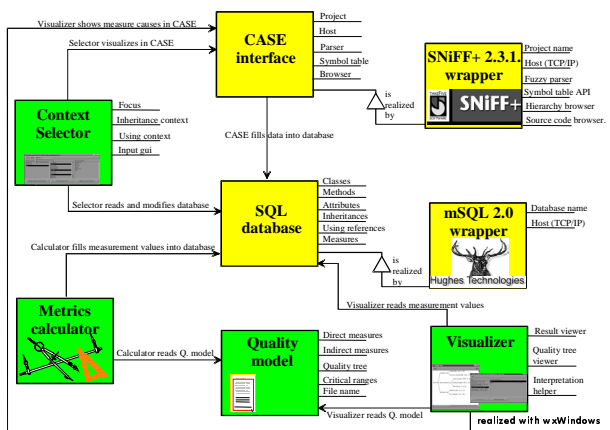
figure 4: Architecture of Crocodile
