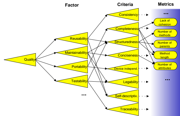
figure 1: Software-quality model
